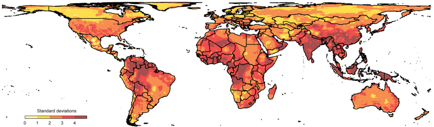
Fig. 6. Projected temperature change by 2050 as a multiple of the local historical standard deviation ( \sigma ) of temperature. Temperature projections are for the A1B scenario and are averaged across 21 global climate models reporting in the CMIP3 (96). Changes are the difference between projected annual average temperature in 2050 and average temperature in 2000. The historical standard deviation of temperature is calculated from annual average temperatures at each grid cell over the period 1950-2008, using University of Delaware data (131). The map is an equal-area projection.
